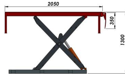
MAXIMUM POSITION OF SCISSOR LIFT
