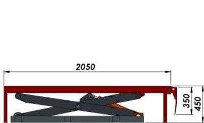
MINIMUM POSITION OF SCISSOR LIFT
