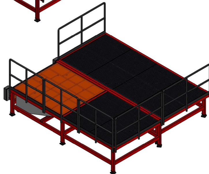
HYDRAULIC LIP DOCK LEVELER
