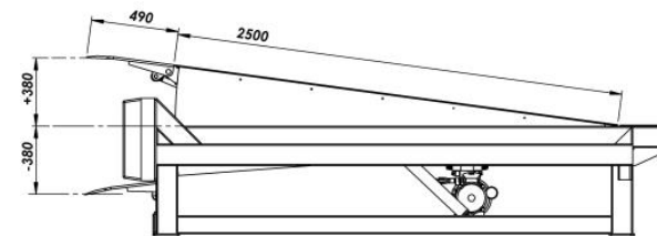
HINGED LIP DOCK LEVELER WORKING RANGE
